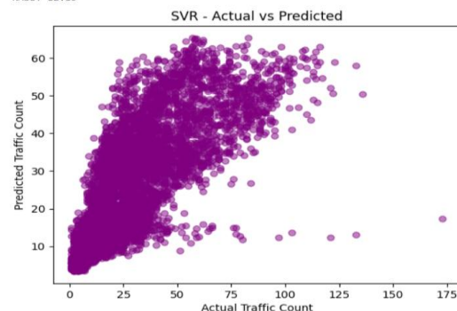
Figure 5: Support Vector Regressor
